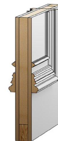
Solid Raised Moulding Profile
