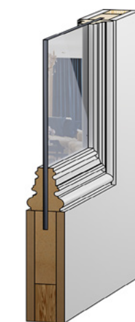
Sunken Moulding Profile with Glass
