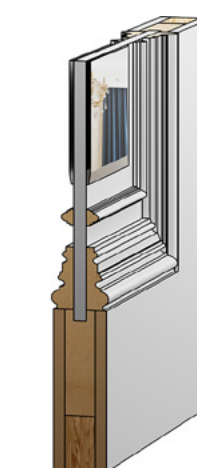
Sunken Moulding Profile with Mirror
